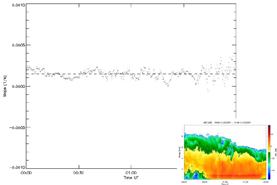
Figure 7. Time series for the vertical mean velocity gradient in a cloud (March 2007). The dots represent single estimates and the dashed line indicates the mean value along the observation period. The reflectivity of the same event is showed in the panel.
