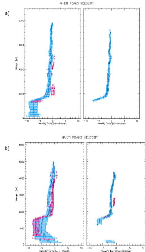
Fig. 3. Examples of mixed-phase spectra profile from data collected on May [a] and March [b] 2007. See text for details.
