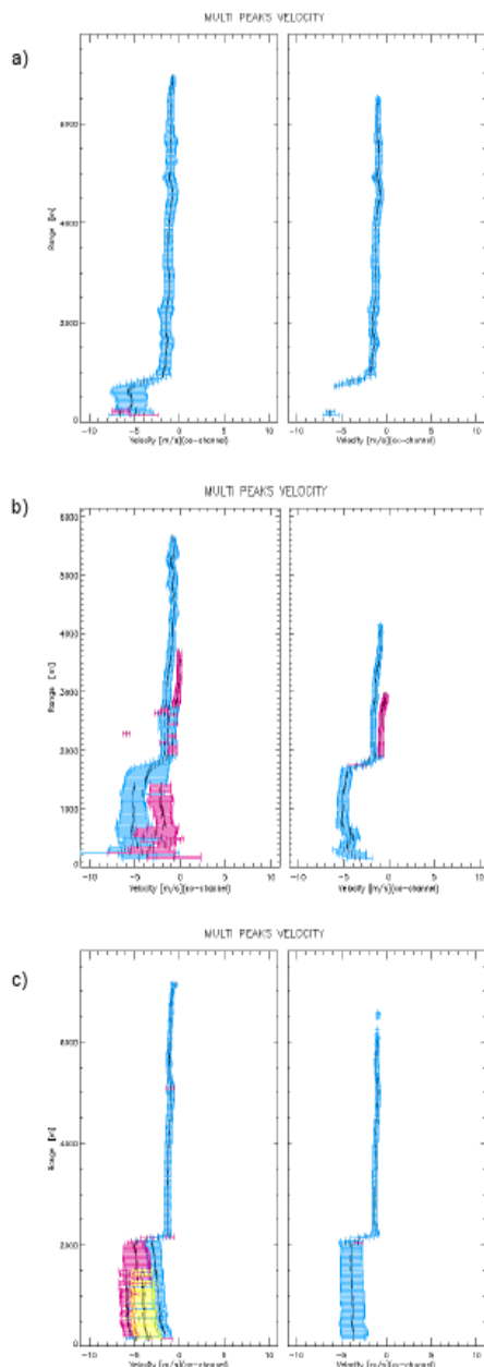
Fig. 2. Examples of Doppler spectra profile from data collected on January [a, b] and March [c] 2007. The resolution is 30 m in range and 10 s in time. Co- and cross-channels are shown for every dwell.
