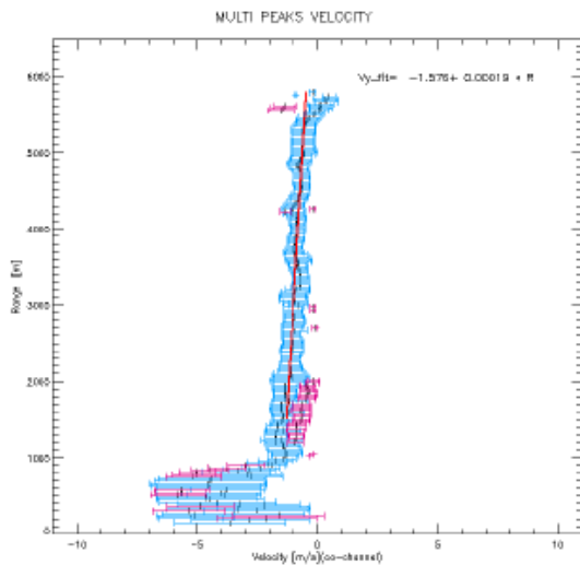
Fig. 6. Examples of spectra profile (March 2007). The mean velocity values for the main cluster in cloud are linearly fitted (red line).
