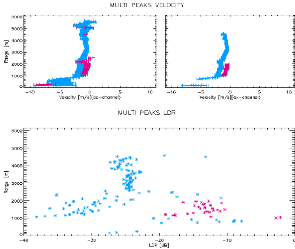
Fig. 5. Example of LDR values for a bimodal spectra profile (February 2007).
